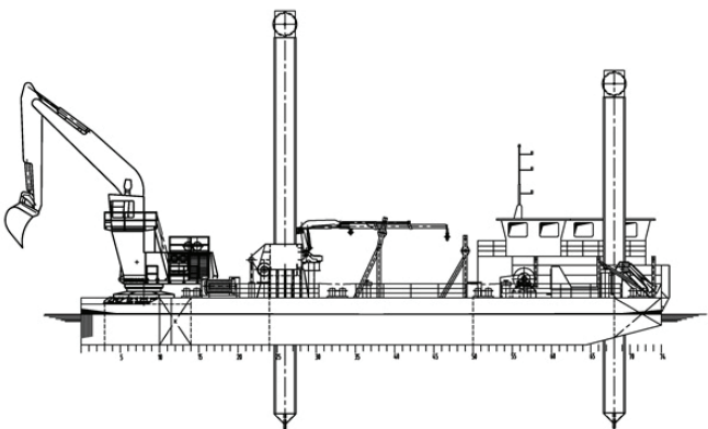
Backhoe dredger (Source: Van Loon Maritime Services).
