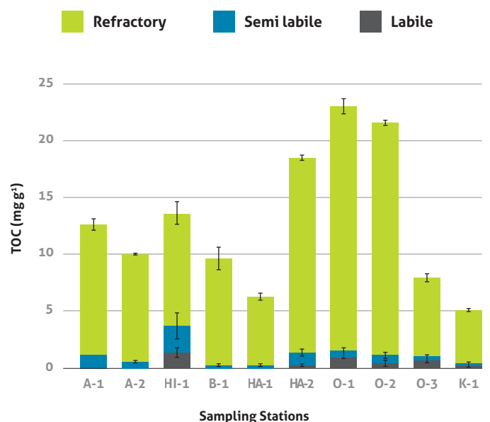
Figure 2.11: Degradation state of coastal sediments in the Osai Inner Sea Japan show how low the percentage of labile organic matter can be. Most of the refractory organic matter consists of humins (Source: Asaoka et al. 2020).
